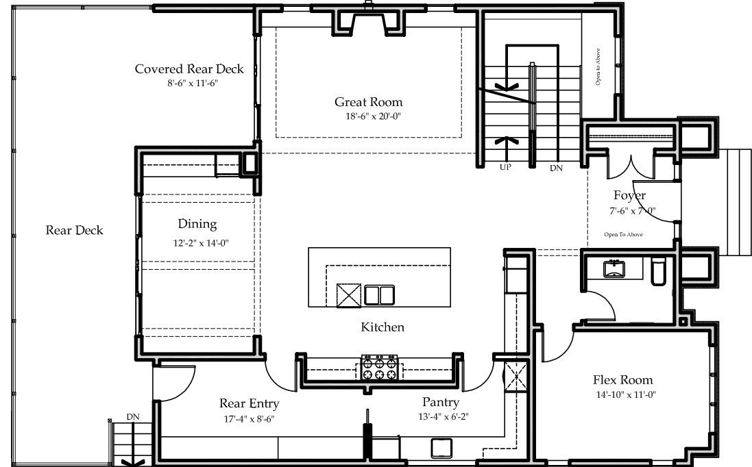
MAIN FLOOR PLAN @ 1,644 SQ.FT. TOTAL AREA: 3,200 SQ.FT.
