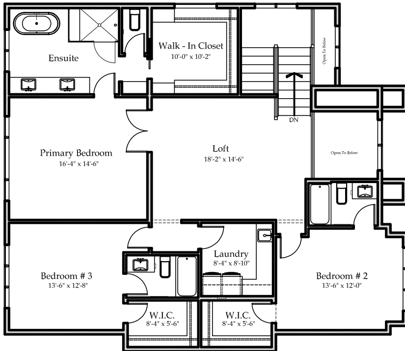
UPPER FLOOR PLAN @ 1,556 SQ.FT.
